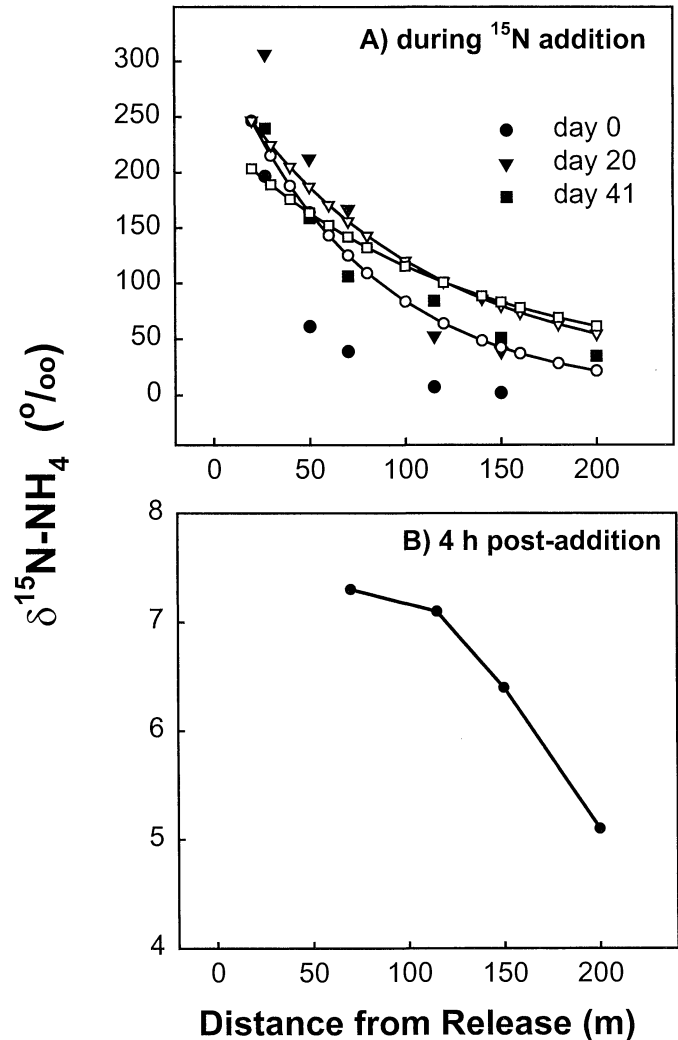
Fig. 2. (A) Longitudinal profile of observed (solid symbols) vs. predicted (open symbols) decline in \delta^{15}\text{NH}_4 on days 0, 20, and 41 of the tracer addition. (B) Observed longitudinal profile of \delta^{15}\text{NH}_4 4 h after the tracer addition stopped on day 42.
