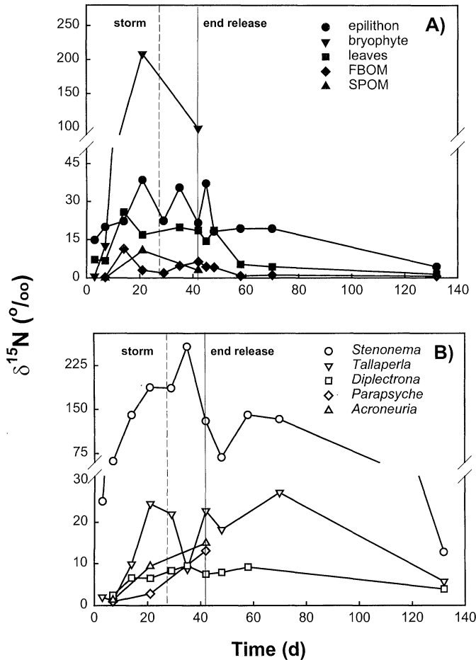
Fig. 5. Time series of observed \delta^{15}\text{N} values at 27 m for the (A) primary uptake compartments, and (B) consumers. The dotted line marks the storm on day 27 and the solid line marks the end of the tracer addition on day 42.
