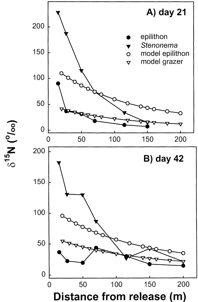
Fig. 4. Longitudinal profile of observed (solid symbols) vs. predicted (open symbols) decline in \delta^{15}\text{N} values of epilithon and the grazing mayfly Stenonema on (A) day 21 and (B) day 42 of the tracer addition.
